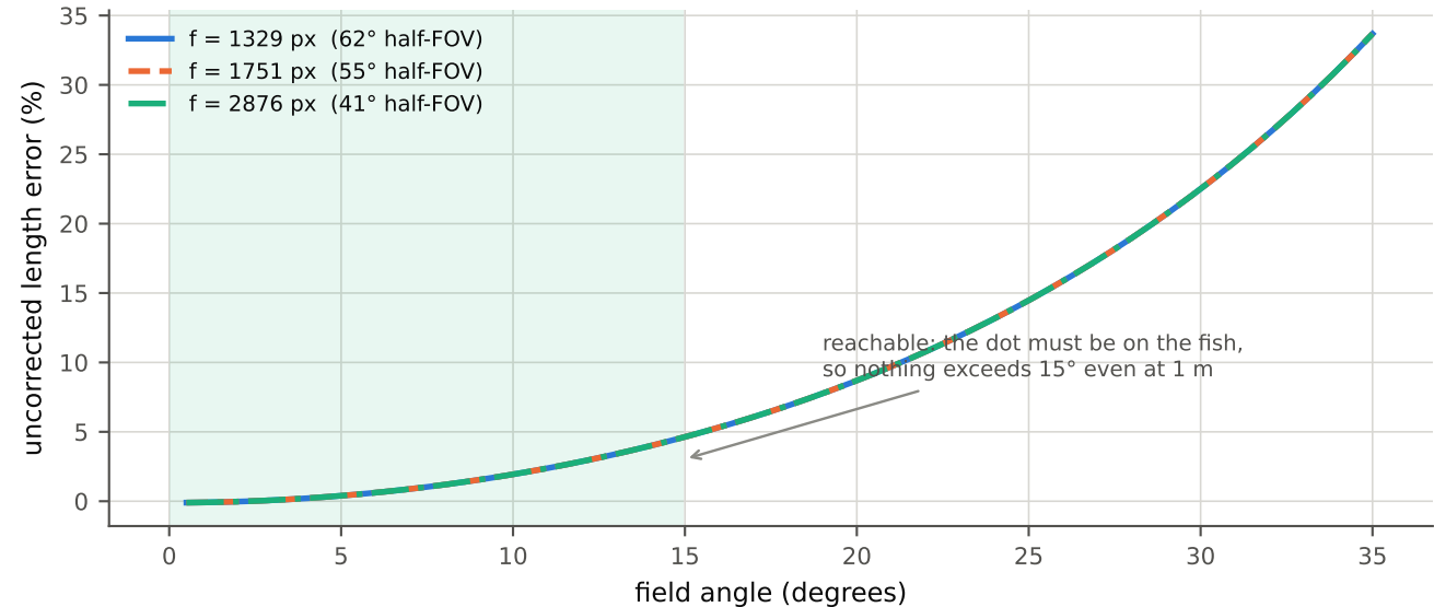
A flat port's error follows the field angle, not the lens
