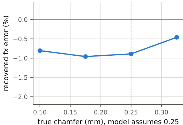
A constant we only think we know
