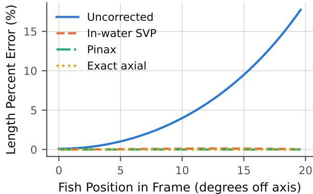
Length Error vs Field Position (0.3 m fish at 2.0 m)
