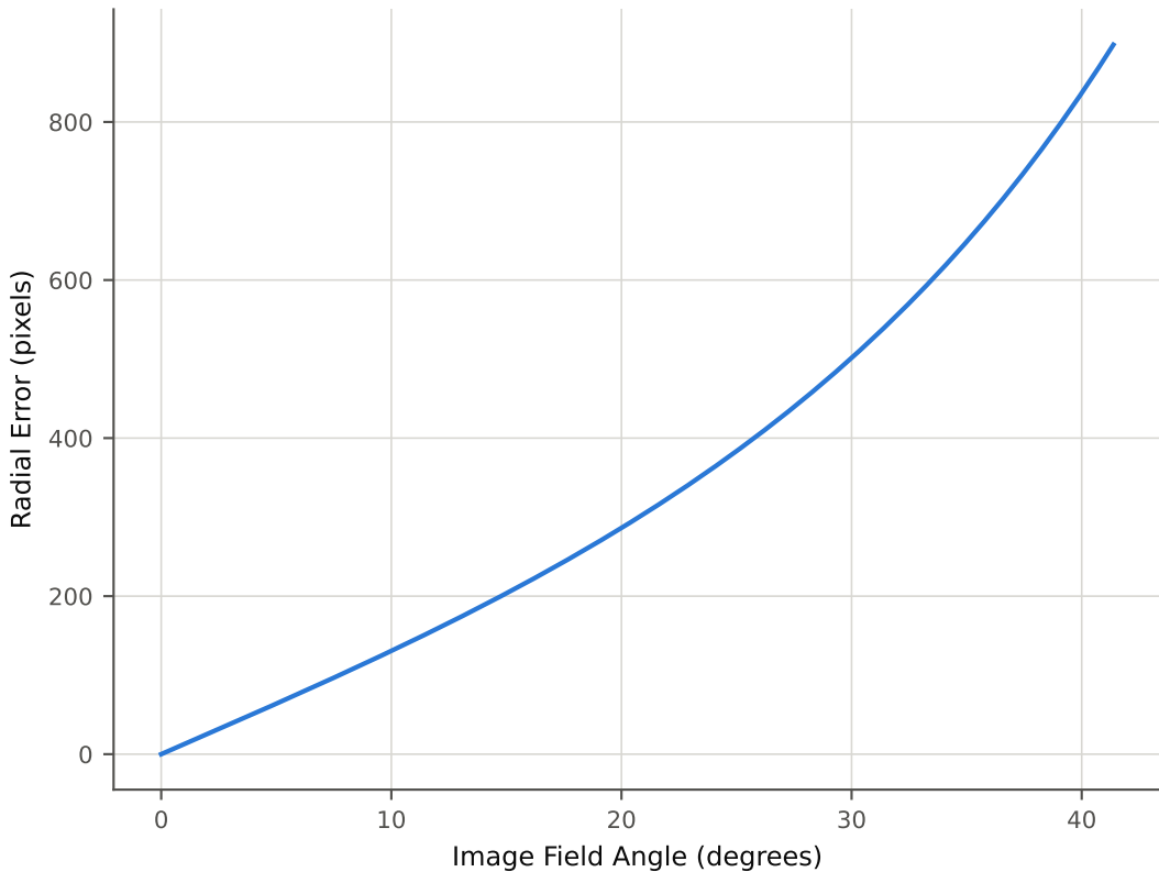
Uncorrected Radial Error at the Image Plane (2 m, salt water)
