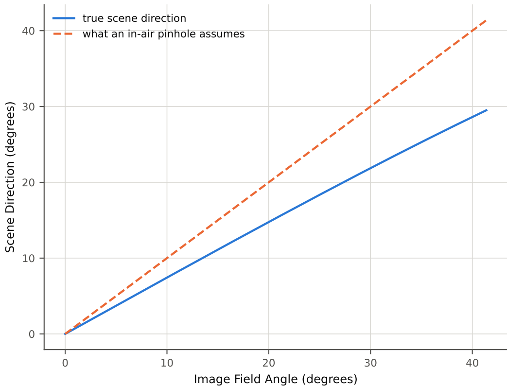
Flat-Port Angular Compression (2 m, salt water)
