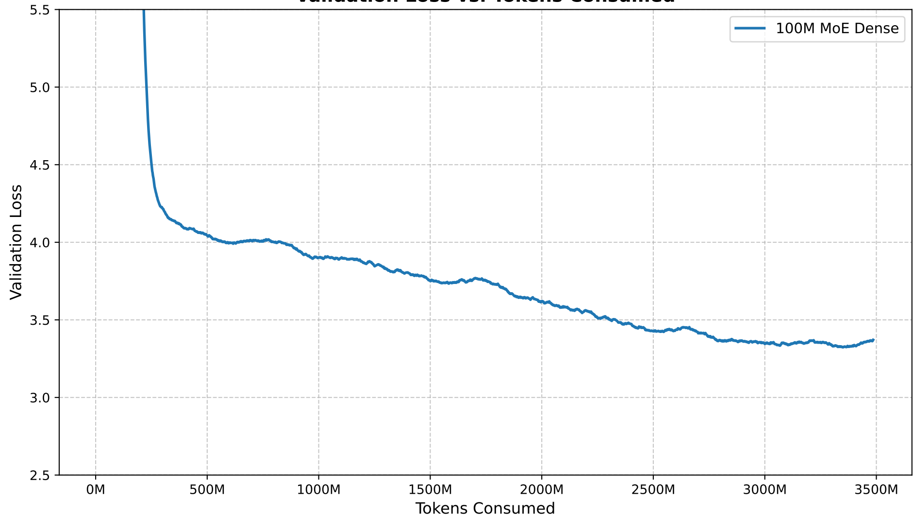
Validation Loss vs. Tokens Consumed
