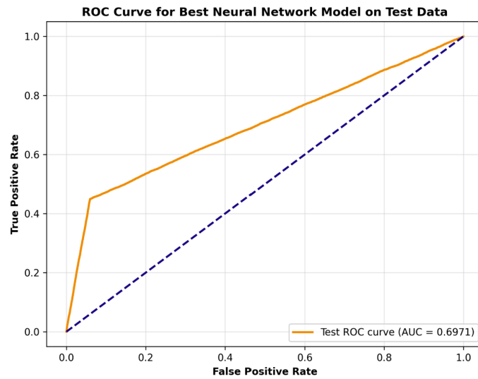
Figure 4. ROC Curve for Best Regular Neural Network Model
