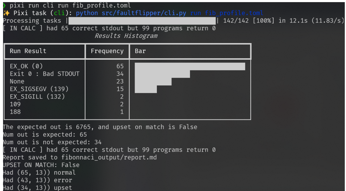
Fig. 12: Success run of our tool with Fibonacci program (1-NOP)
