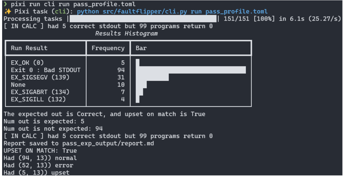
Fig. 6: Success run of our tool with Password Check program
