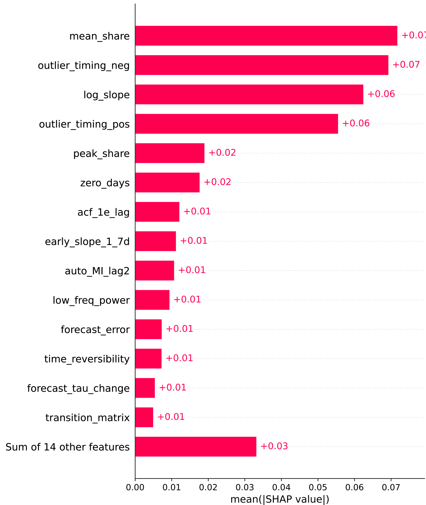
Global feature importance
