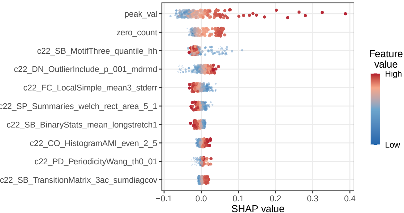
SHAP Beeswarm (Top 10 Features)
