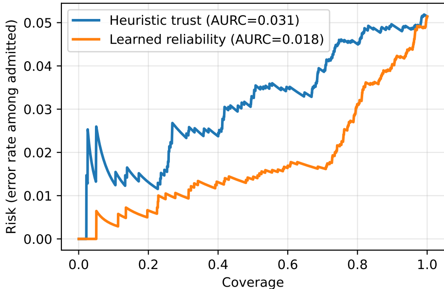
Risk-coverage — held-out CORAL test (Gemma-4 ensemble)
