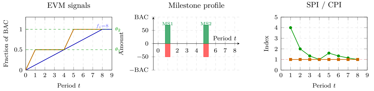
Figure 7: SP-4 project view (single-project). Outcome: completed . Z^* = 36.29 .
