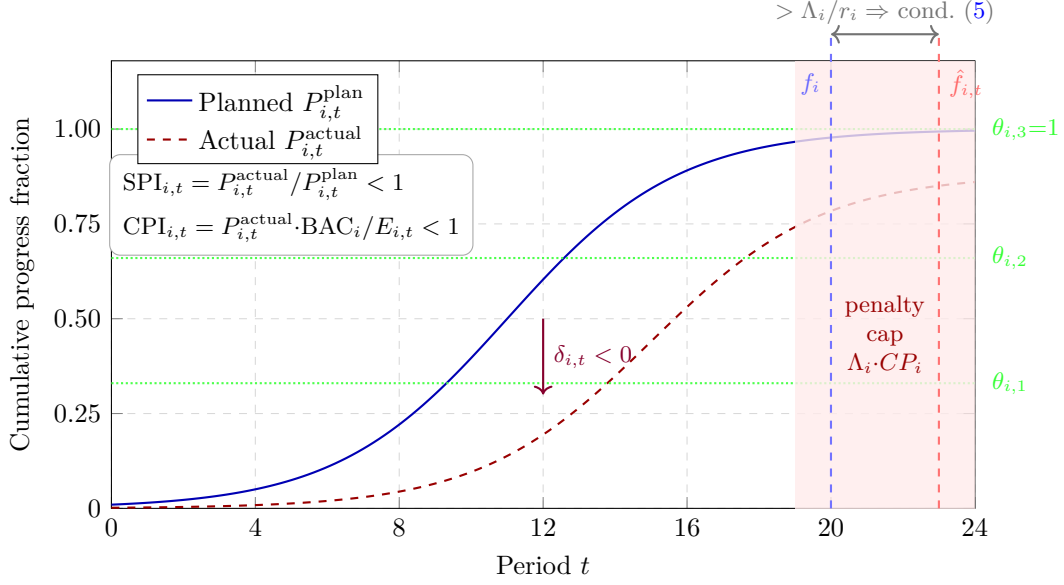
Figure 4: S-curve expenditure profile with EVM signals for a lagging project. The planned curve follows the regularized incomplete Beta function; actual progress runs below, producing negative signed deviation \delta_{i,t} and values SPI_{i,t}, CPI_{i,t} < 1 . Dashed horizontals mark milestone thresholds \theta_{i,j} . When the forecast finish gap \hat{f}_{i,t} - f_i exceeds \Lambda_i/r_i (shaded region), Termination Condition (5) activates.
