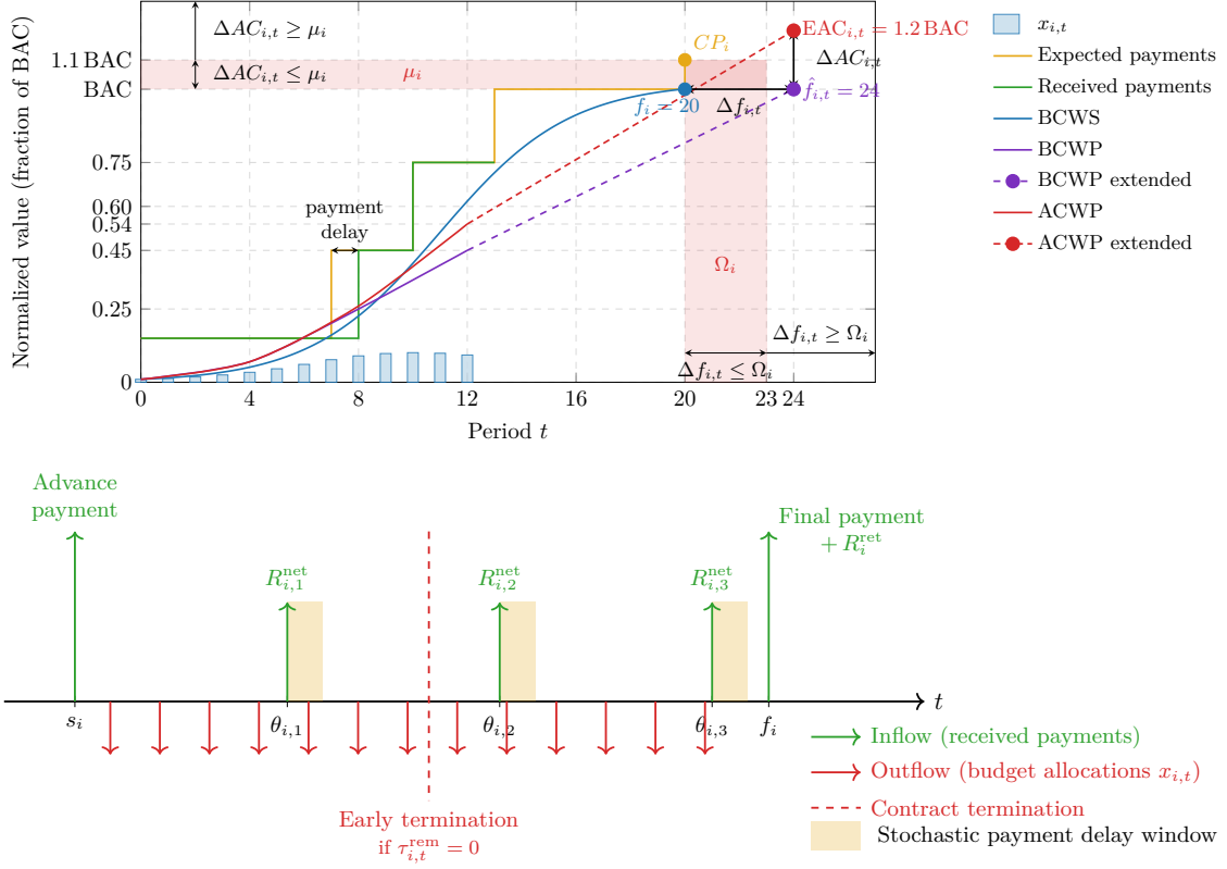
Figure 3: EVM-based termination conditions (top) and per-project payment profile under FIDIC contract mechanics (bottom).
