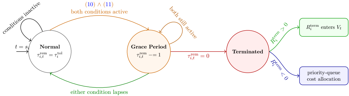
Figure 6: Finite-state representation of the termination mechanic for project i .
