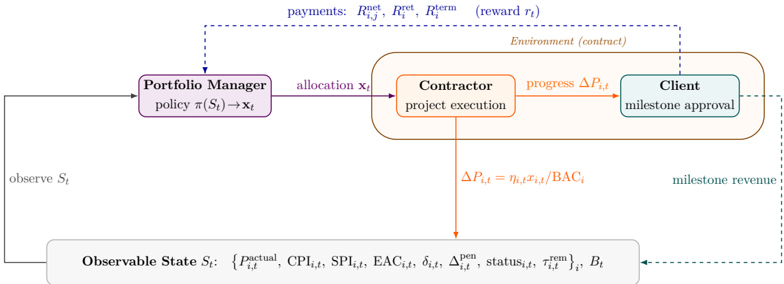
Figure 4: Portfolio governance as a reinforcement learning feedback loop.
