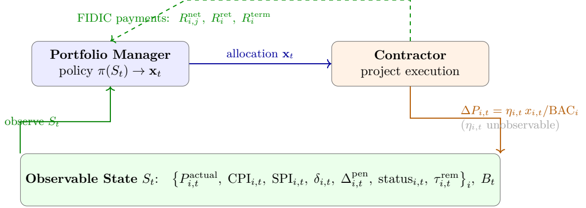
Figure 1: Portfolio governance feedback loop. The portfolio manager (agent) controls only the budget allocation vector \mathbf{x}_t . Contractors convert allocations into physical progress through efficiency \eta_{i,t} , which is unobservable and realized only after commitment. The full state S_t is observable each period; FIDIC milestone payments, retention release, and termination settlement flow back as cash inflows.
