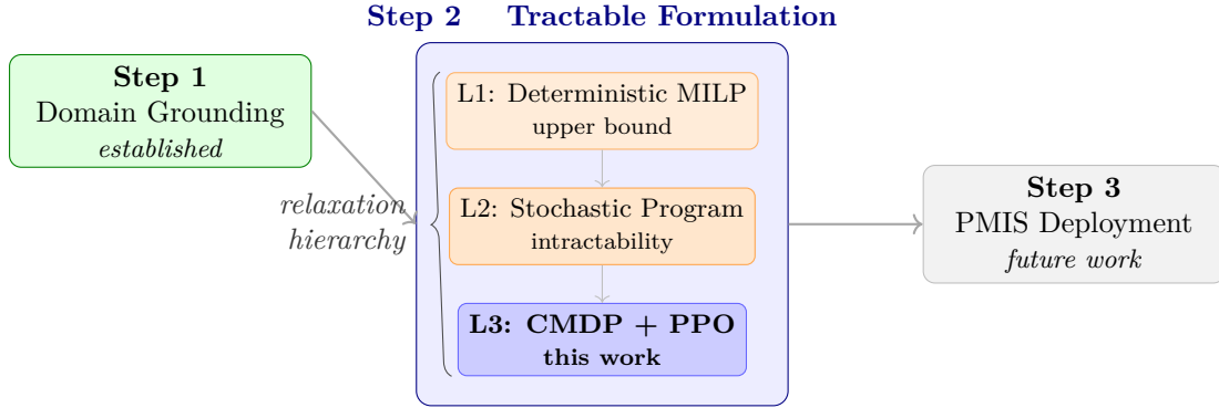
Figure 3: Solution maturity progression toward deployable portfolio-level budget allocation.
