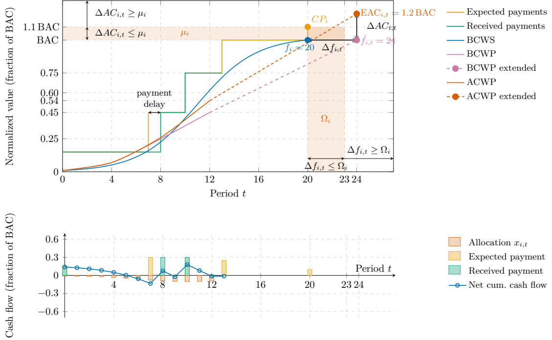
Figure 3: EVM-based termination conditions (top) and periodic project cash flow profile (bottom): payments received above zero, budget allocations below zero, net cumulative cash flow line.
