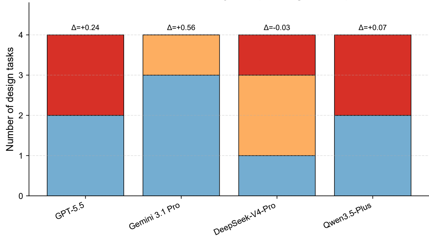
BEAVER win/tie/loss by task (tie margin = 0.10)
