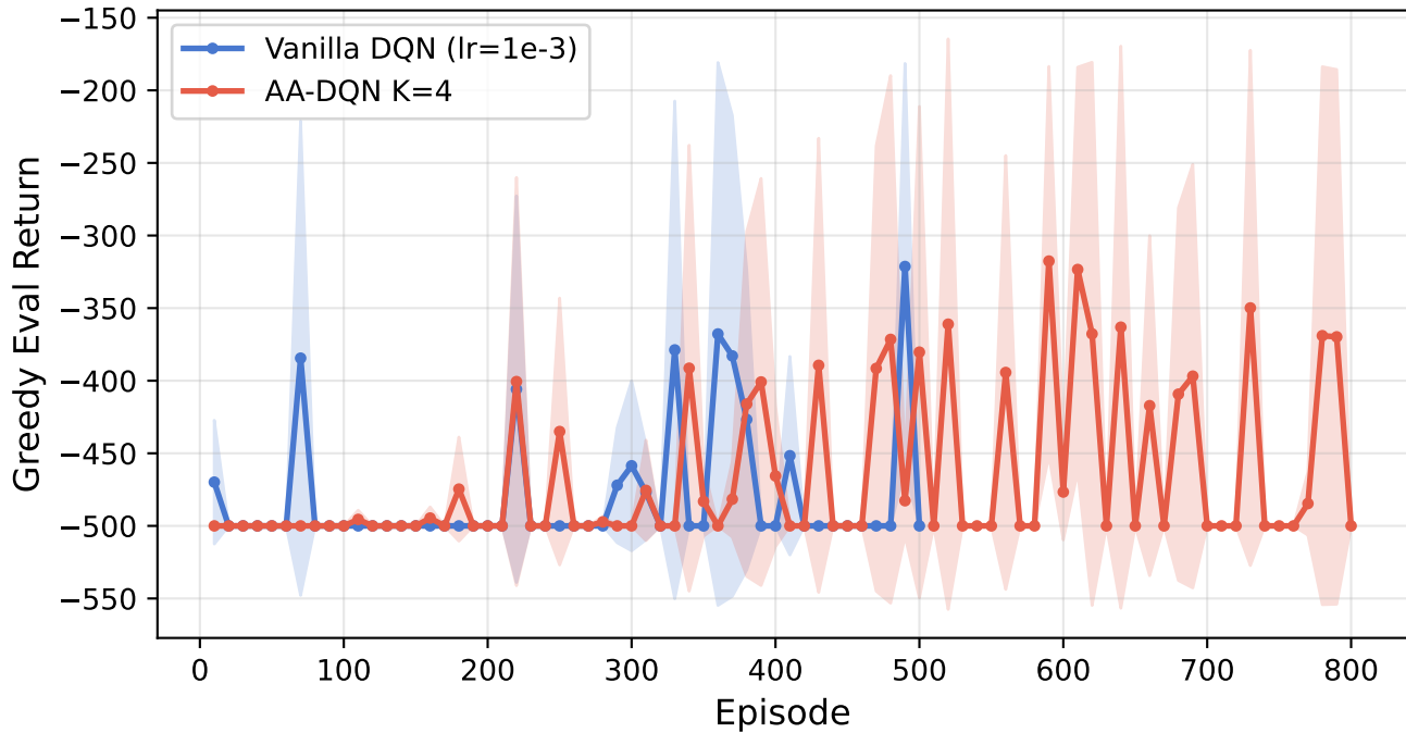
Evaluation Returns on Acrobot-v1 (mean \pm std, 3 seeds)
