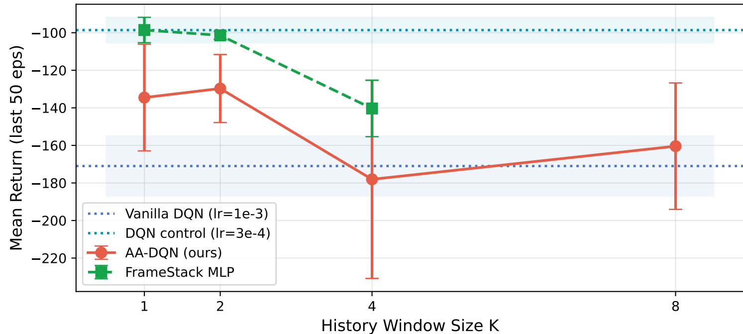
K Ablation: AA-DQN vs FrameStack vs DQN Baselines on Acrobot-v1
