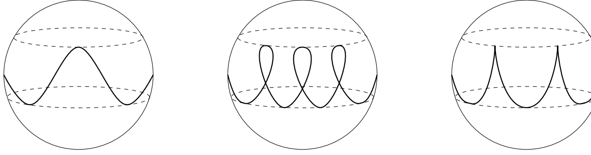
Figure 33: From left to right, monotone precession, spin-reversal precession and non-monotone precession.
