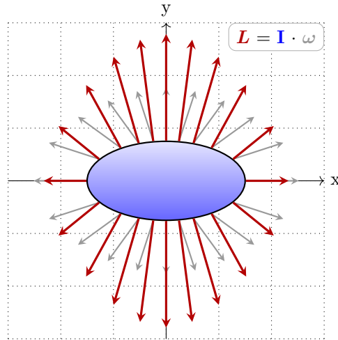
Figure 32: Graphical representation of the relationship between the angular velocity vector \omega (gray) and the angular momentum vector \mathbf{L} (red) for an ellipsoid with inertia tensor \mathbf{I} . The directions of \mathbf{L} and \omega do not coincide due to the anisotropy of the inertia tensor. The ellipsoid has dimensions 3, 1.5 and 1.5 along the x, y, and z axes respectively and is homogeneous in density.
