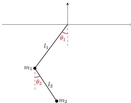
Figure 2: Double pendulum.
