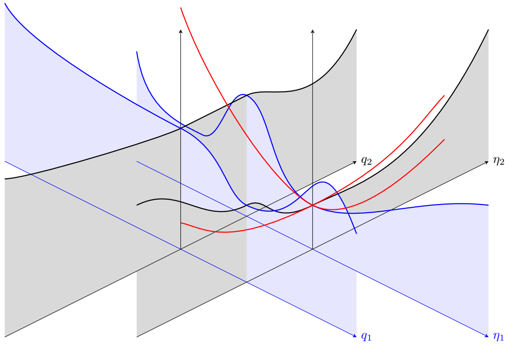
Figure 36: Expansion around a small diversion in a minimum up to second order.
