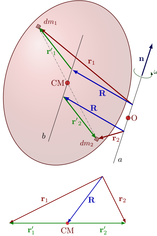
Figure 30: One wants to prove that I_a = I_b + M(\vec{R} \times \vec{n})^2 . For this, one can consider the 3D figure. Notice that all vectors in green, blue and red are perpendicular to the vector \vec{n} . For a point-symmetrical, homogeneous body, it is enough to show that for two point masses dm_1, dm_2 , dI_a = dI_b + dI_{CM} . Here, dI_a = dm_2 r_2^2 + dm_1 r_1^2 = dm_1(r_1^2 + r_2^2) , dI_{CM} = 2dm_1 R^2 , and dI_b = 2dm_1 r_1'^2 , as due to homogeneity dm_1 = dm_2 . We then have dI_{CM} + dI_b = 2dm_1(R^2 + r_1'^2) , so for equivalence to hold one needs that r_1^2 + r_2^2 = 2(R^2 + r_1'^2) . This can be interpreted in the 2D triangle of the second figure. One finds this triangle by combining the two smaller triangles in the 3D figure and projecting them on a plane perpendicular to the vector \vec{n} . Notice that, as masses dm_1 and dm_2 were chosen symmetrically with respect to the CM, one has r_1' = r_2' . The relation r_1^2 + r_2^2 = 2(R^2 + r_1'^2) then trivially holds due to Apollonius's theorem.
