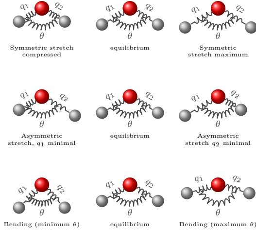
Figure 34: Vibrational modes of \text{H}_2\text{O} : 3N=9 degrees of freedom total. 3 vibrational (shown), 3 translational, 3 rotational. Modes: symmetric stretch ( q_1 = q_2 ), asymmetric stretch ( q_1 \neq q_2 ), bending ( \theta ).
