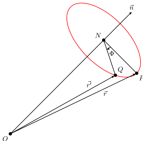
Figure 8: Finite rotation around an axis.
