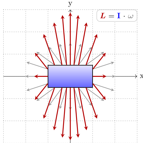
Figure 29: Graphical representation of the relationship between the angular velocity vector \omega (gray) and the angular momentum vector L (red) for a rectangular beam with inertia tensor I . The directions of L and \omega do not coincide due to the anisotropy of the inertia tensor. The rectangular beam has dimensions 2, 1, and 0.2 along the x, y, and z axes respectively and is homogeneous in density.
