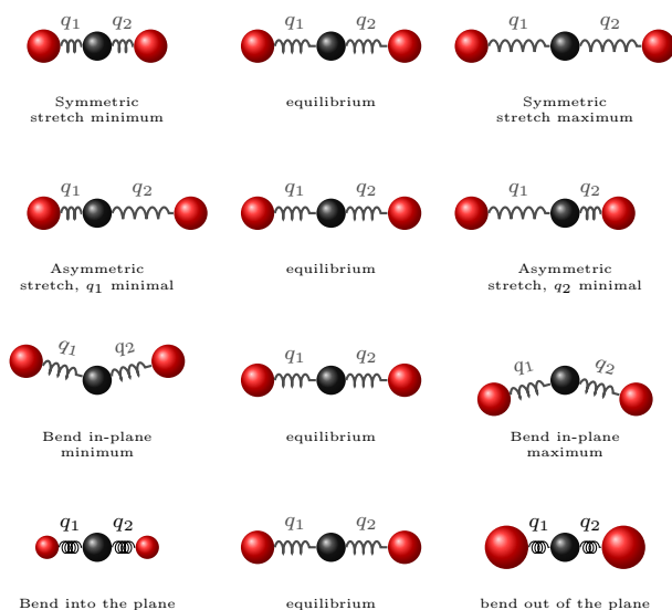
Figure 35: Vibrational modes of \text{CO}_2 : 3N=9 degrees of freedom total. 4 vibrational (shown: symmetric and asymmetric stretch, bending in/out-plane), 3 translational, 2 rotational. Bending doubly degenerate (linear molecule). The springs between the C-O bonds and the corresponding generalized coordinate \theta are omitted to avoid overloading the figure.
