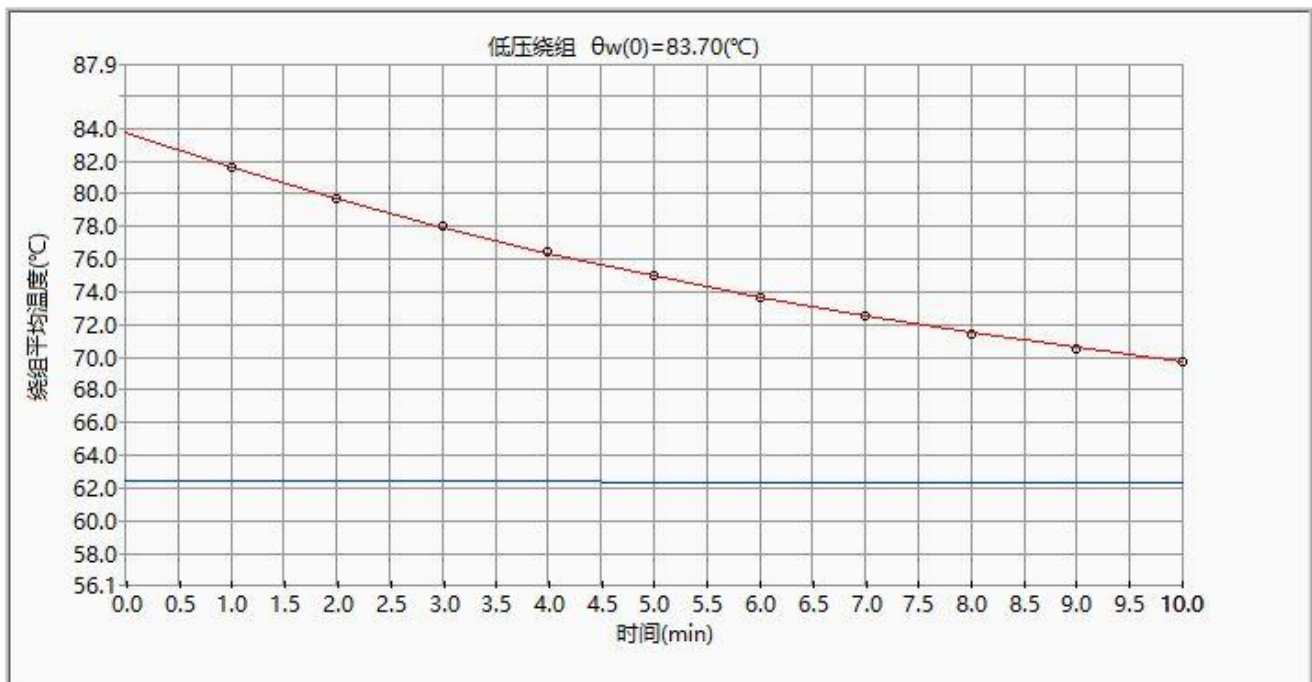
F2 LV winding temperature curve
