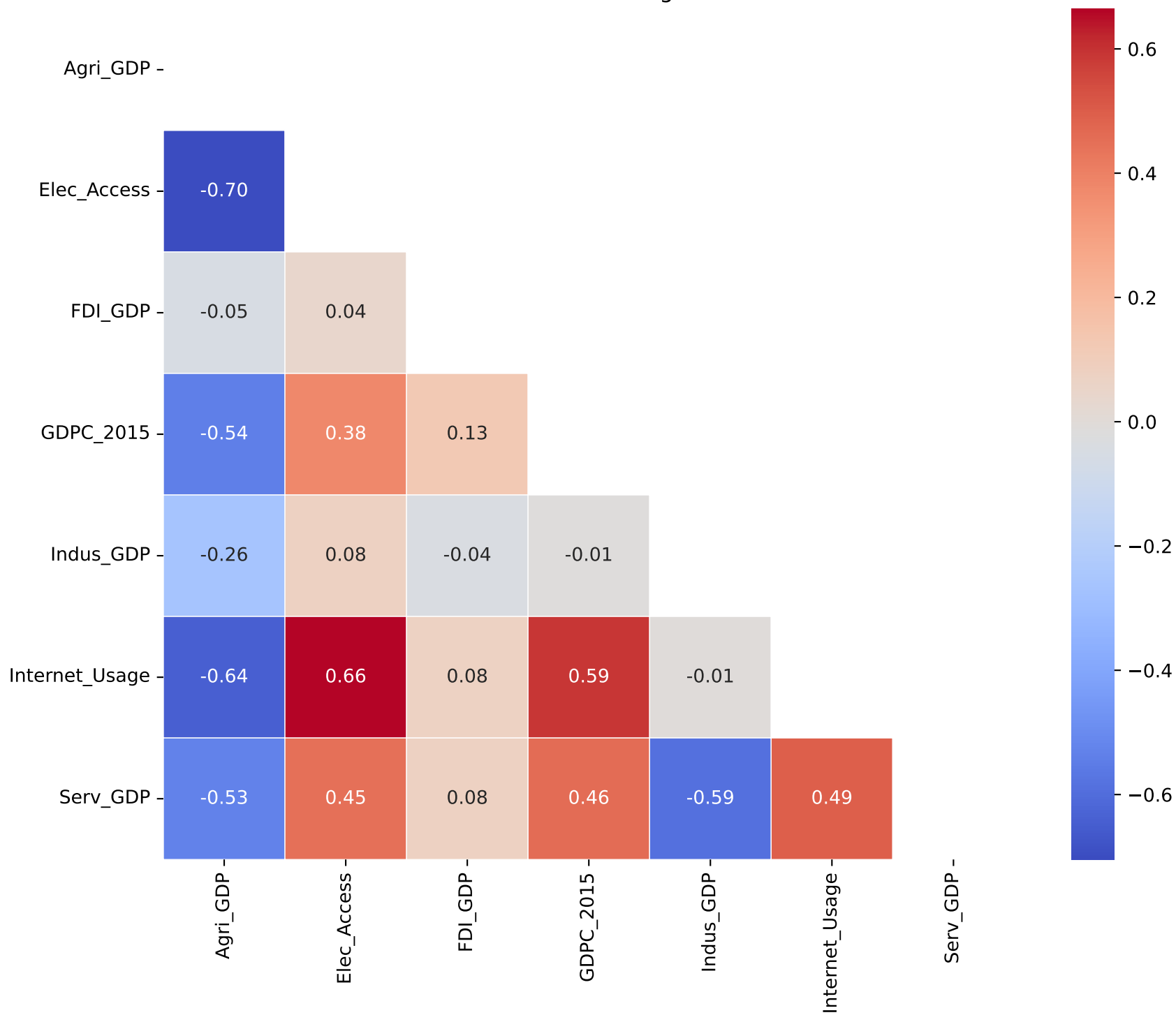
Correlation Matrix - Original Data
