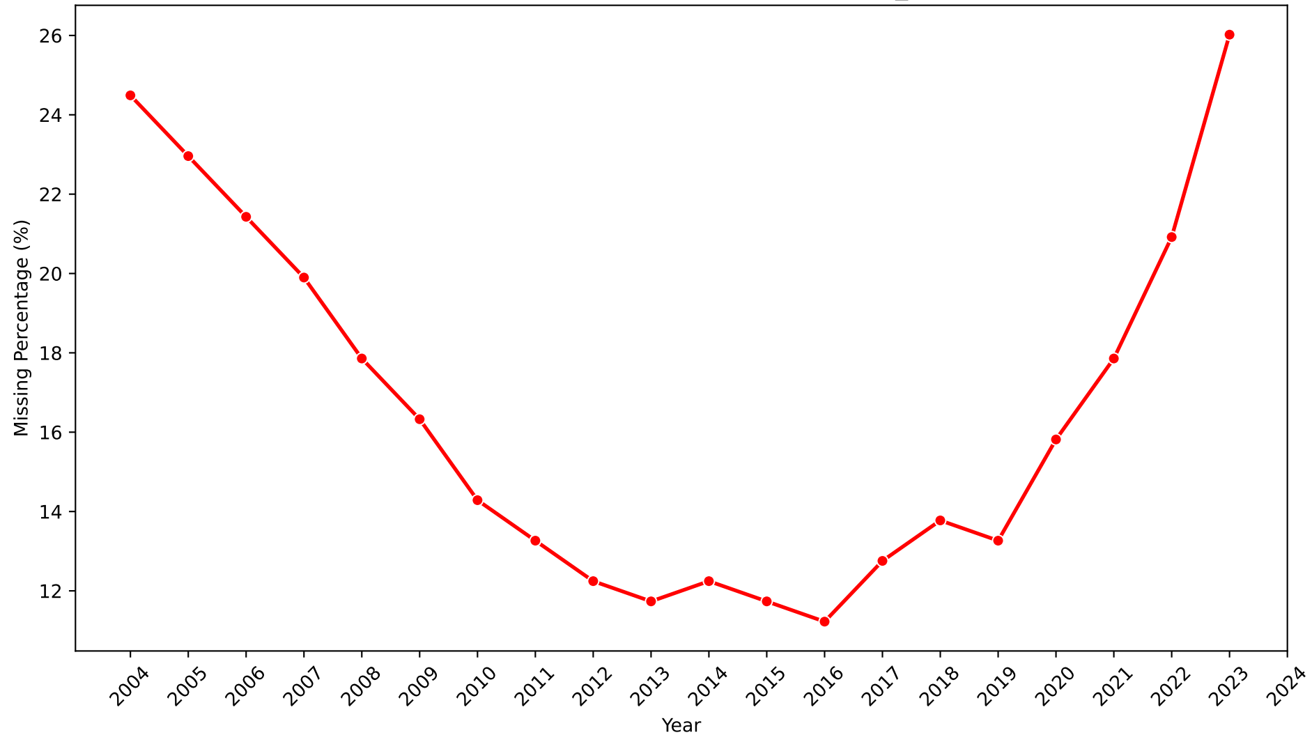
Missing Values Trend by Year - Credit_Private
