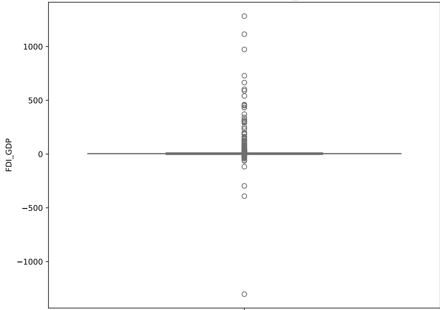
Overall Boxplot - FDI_GDP
