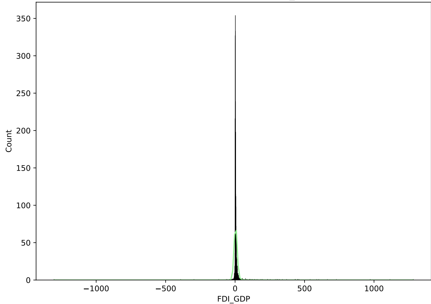
Overall Histogram - FDI_GDP
