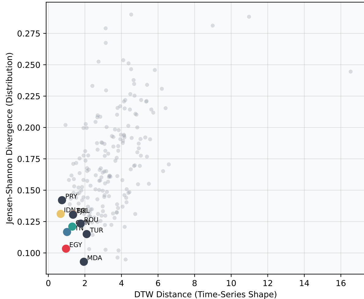
DTW (Vector) vs JSD (Distribution) (Bottom-Left Region = High Similarity in Both Dimensions)
