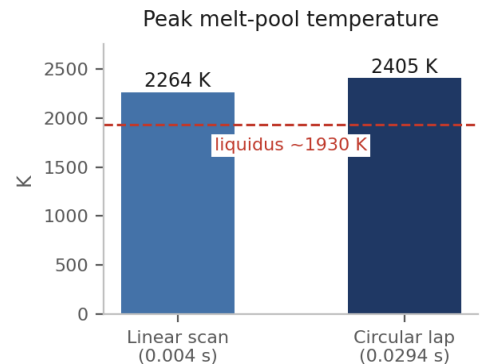
Fig. 4 - Peak melt-pool temperature by scan strategy
