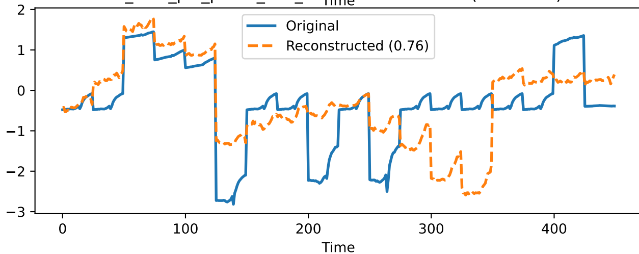
b_field_pol_probe_obv_field Reconstruction (Max Error)
