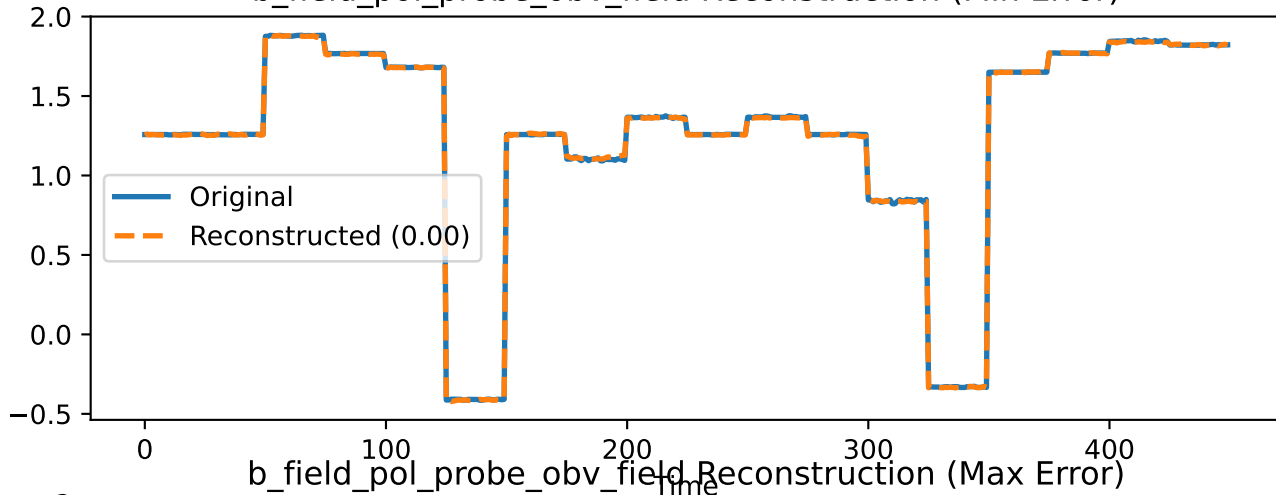
b_field_pol_probe_obv_field Reconstruction (Min Error)
