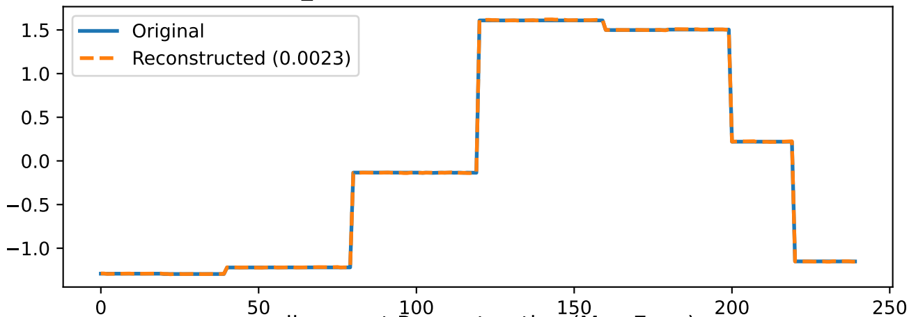
coil_current Reconstruction (Max Error)
