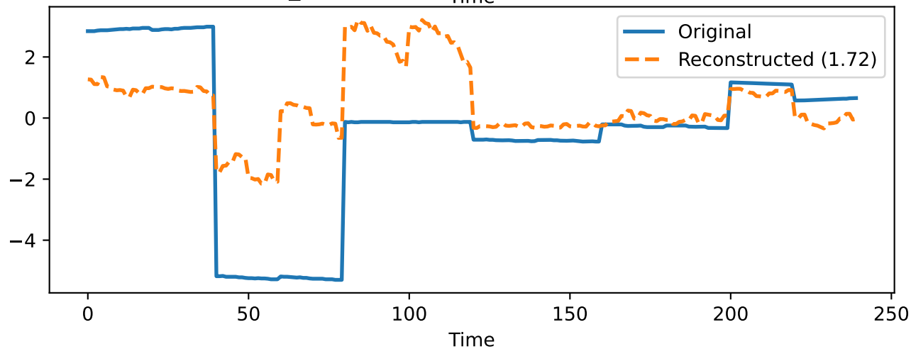
coil_current Reconstruction (Max Error)
