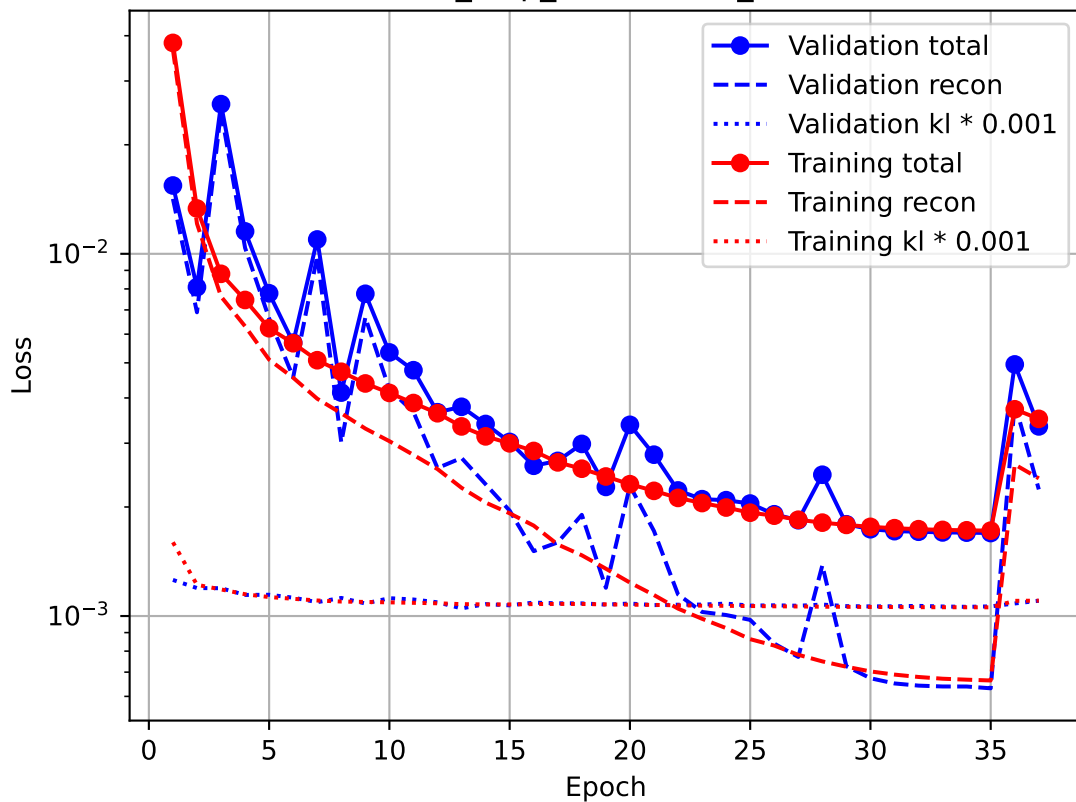
flux_loop_fluxConv1d_VAE
