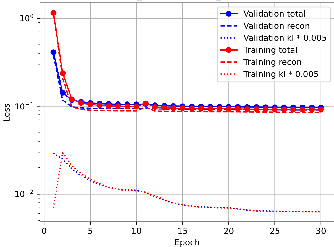
i_plasmaConv1d_VAE
