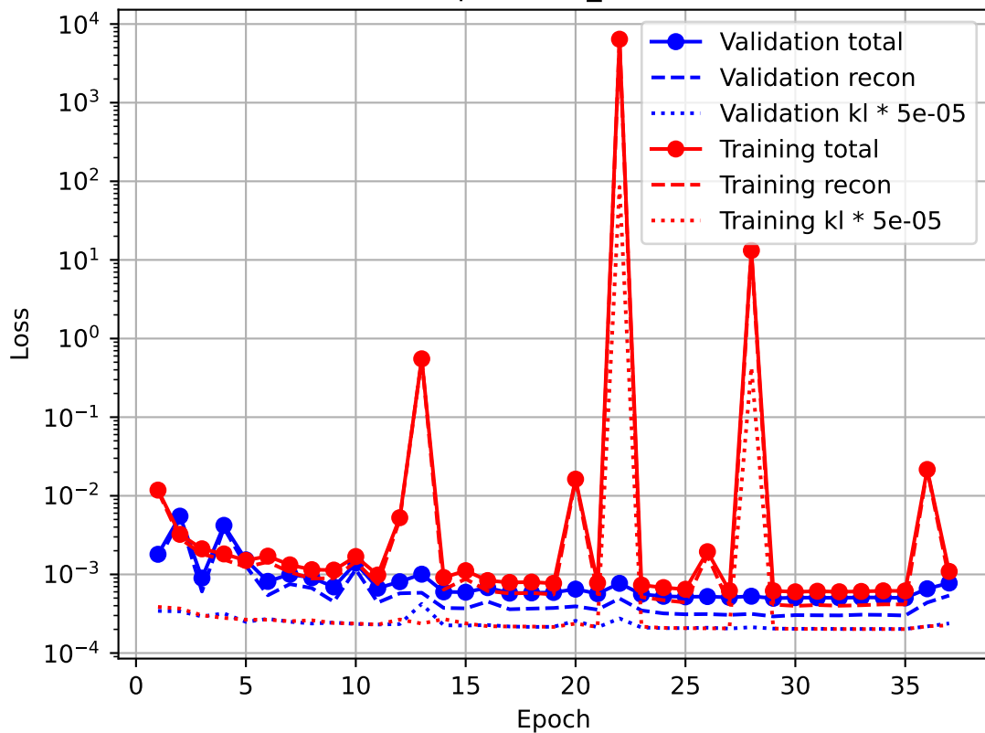
ipConv1d_VAE
