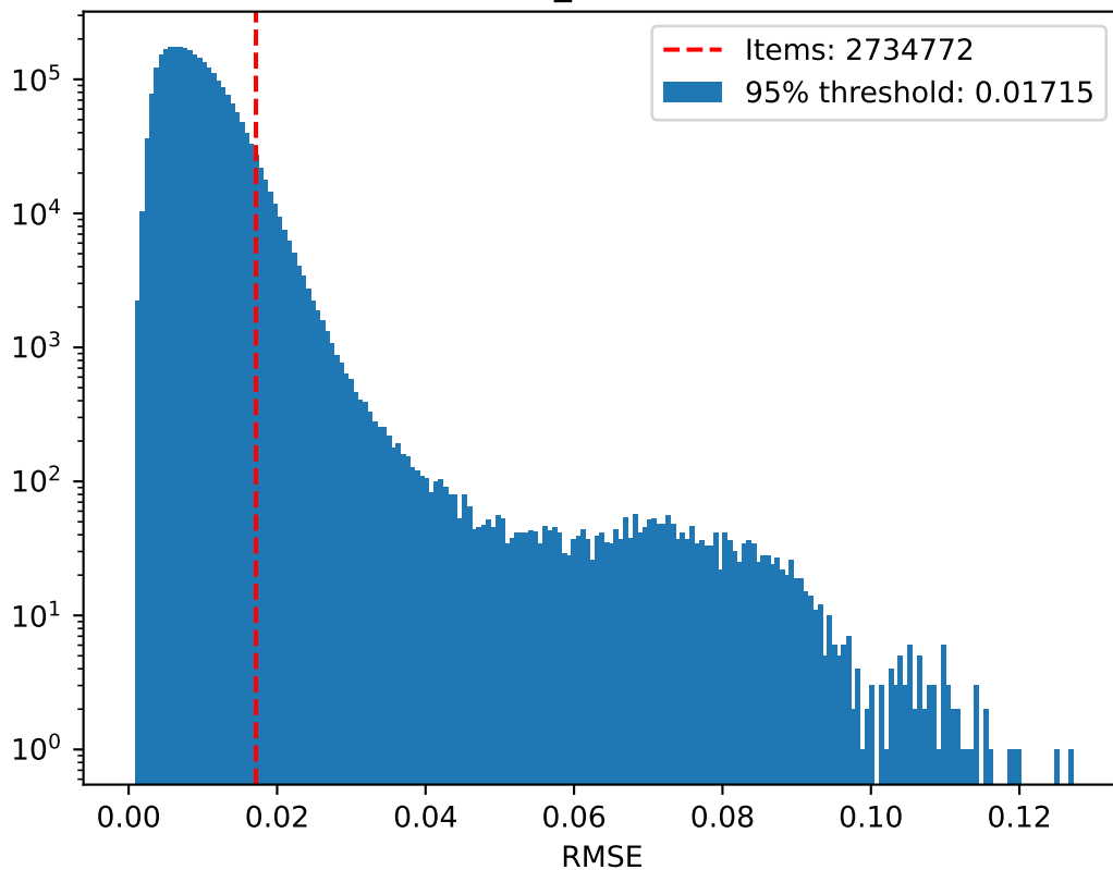
solenoid_currentRMSE
