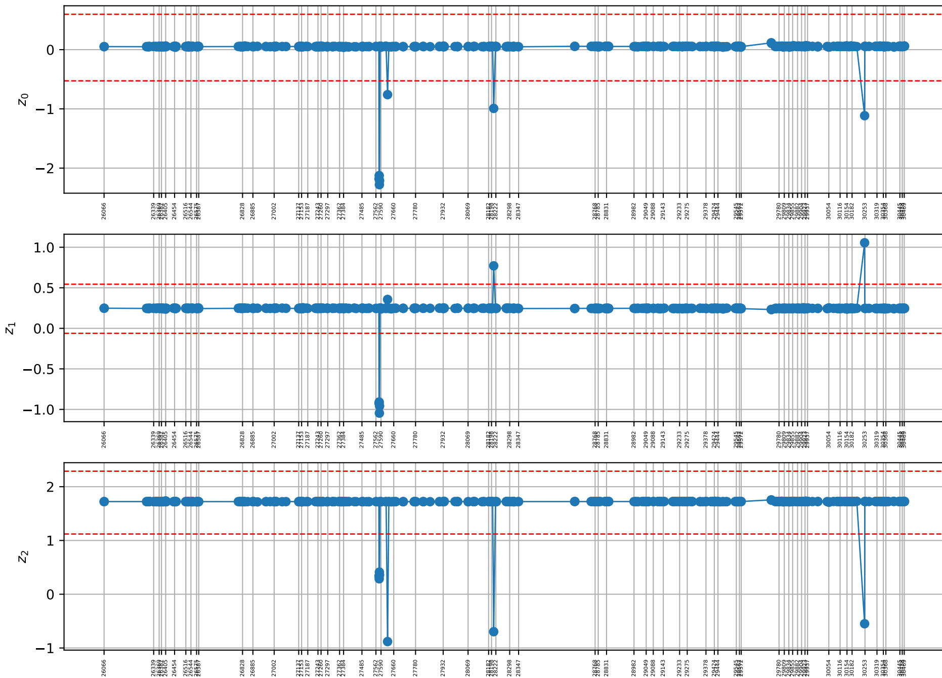
Latent coordinates for window 10
