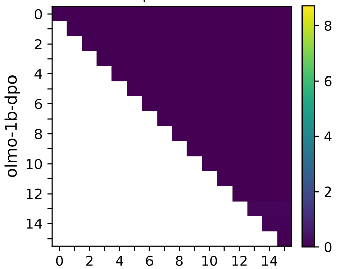
implicatures
