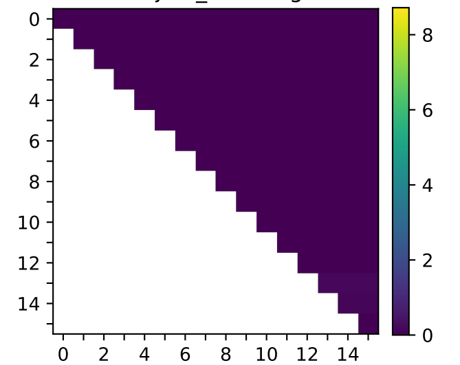
object_counting
