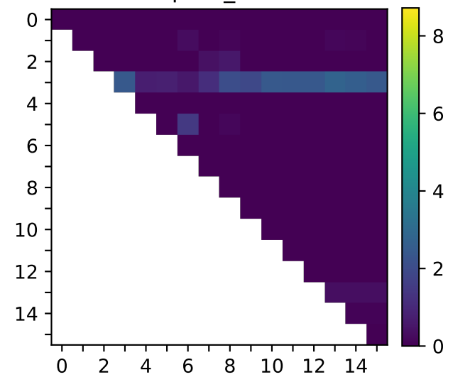
metaphor_boolean
