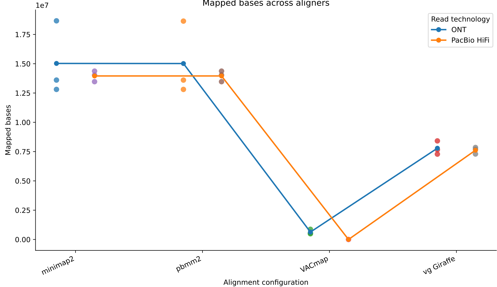
Mapped bases across aligners
