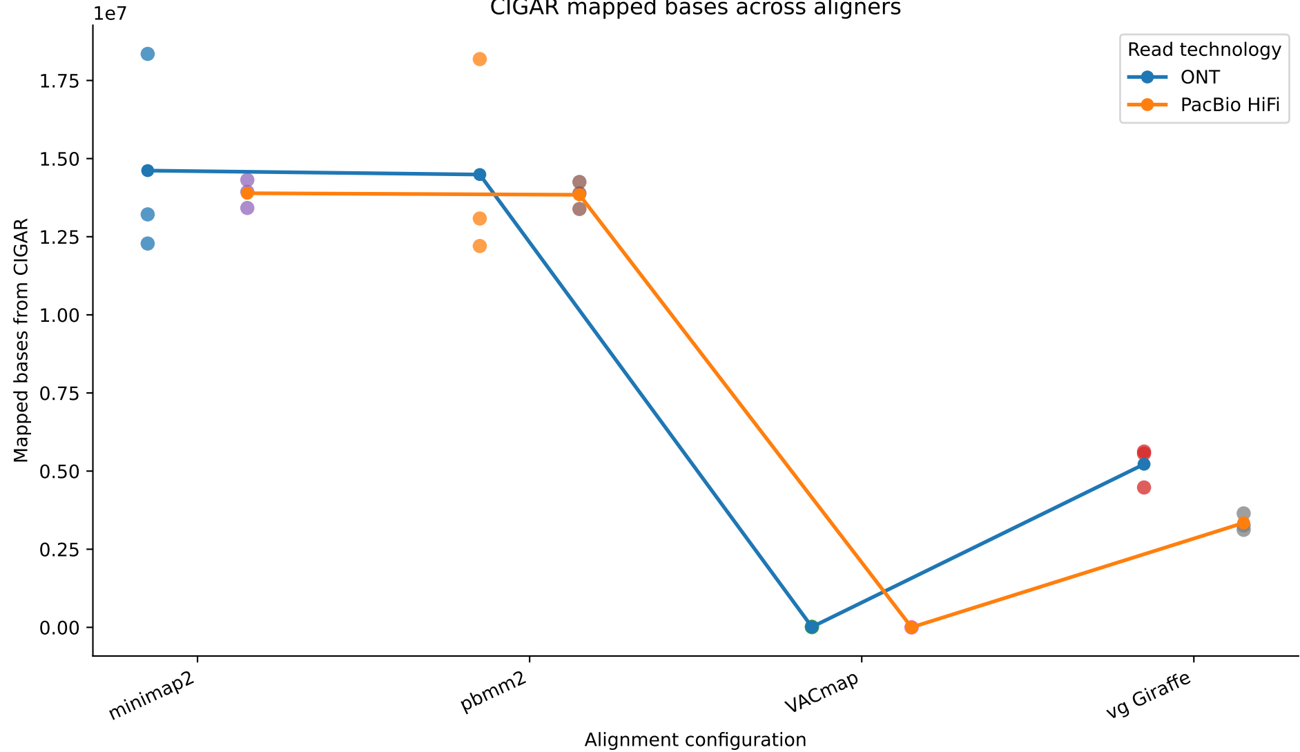
CIGAR mapped bases across aligners
