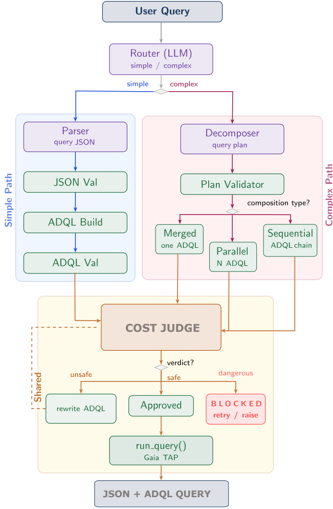
Figure 2. Overview of the proposed pipeline. A router classifies each query as simple or complex and dispatches it to the corresponding path. Both paths converge on a shared cost judge before executing the final ADQL query against the Gaia TAP server.
