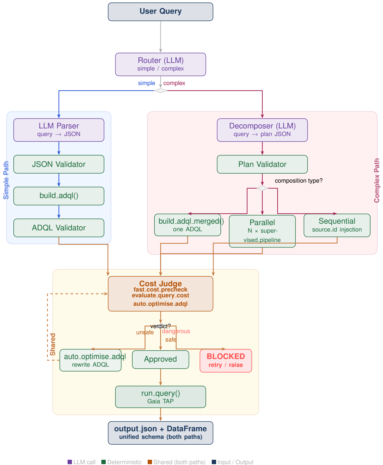
Figure 1. Gaia intelligent query pipeline.
