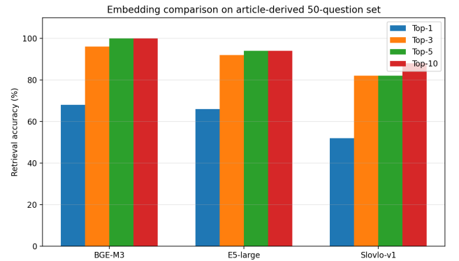
Figure 2. Embedding comparison on the final 50 questions dataset.
