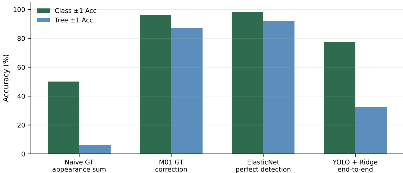
Counting performance gap between perfect and YOLO detections
