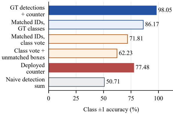
Fig. 2. Detection and aggregation diagnostics: (a) six counting rules; (b) confidence-threshold sensitivity of Ridge+ F_{\text{all}} . Diagnostic rules are separate estimators, not additive error components.
