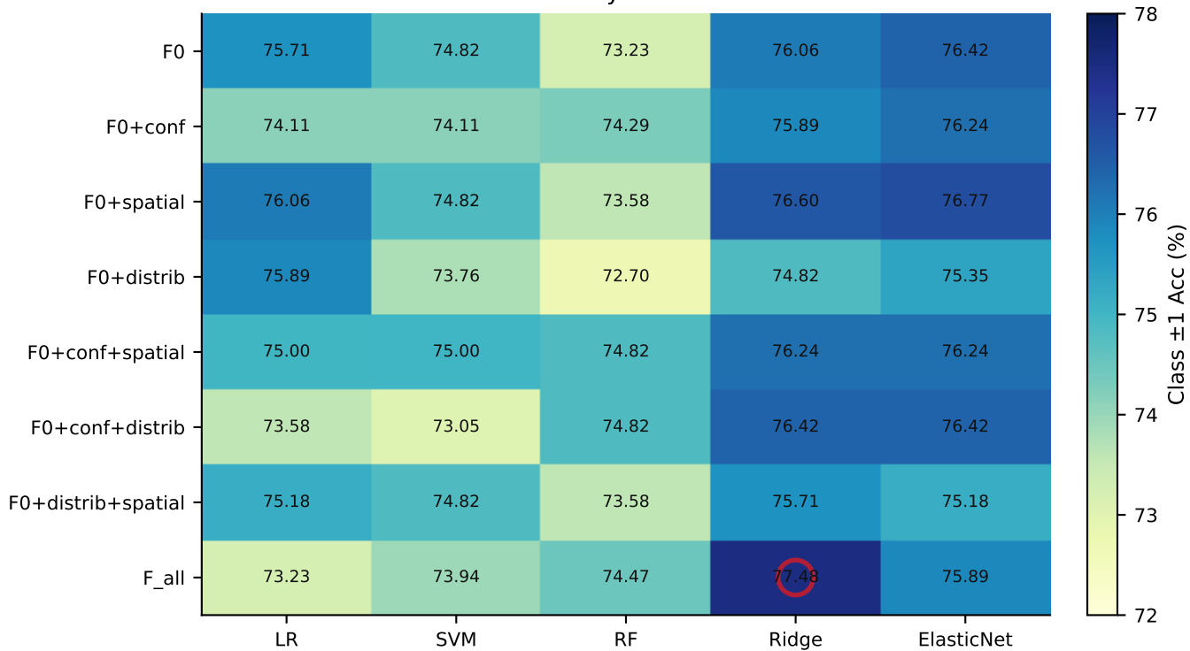
Controlled train-only matrix: Class \pm 1 Acc
