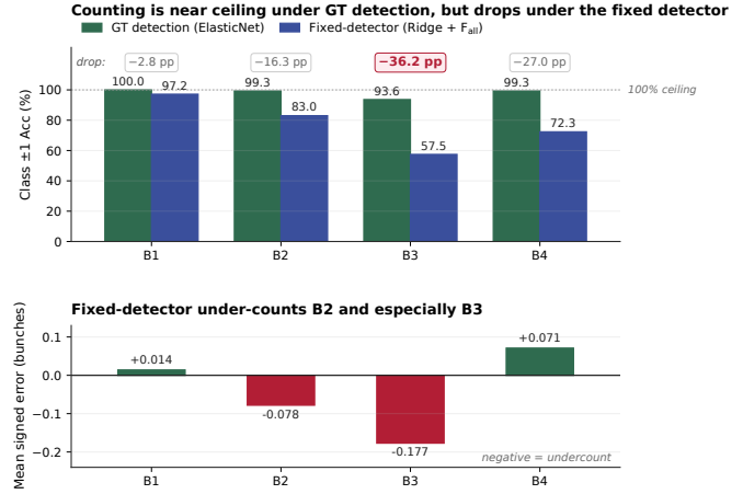
Fig. 3. Top: Per-class Class \pm 1 Acc for the best counter in each detection condition (ElasticNet under GT; Ridge + F_{\text{all}} under the fixed detector). Counting is near ceiling under GT detection but drops sharply under the fixed detector. Bottom: Per-class signed bias of Ridge + F_{\text{all}} in the fixed-detector setting. Negative values indicate systematic under-counting; the under-count is concentrated on B2 and especially B3.
