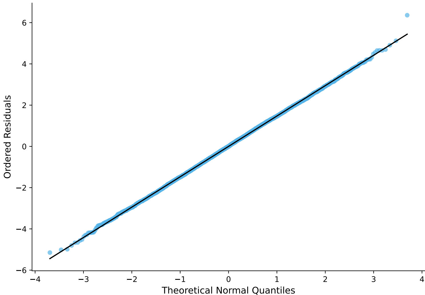
Normal Q-Q Plot of Residuals
