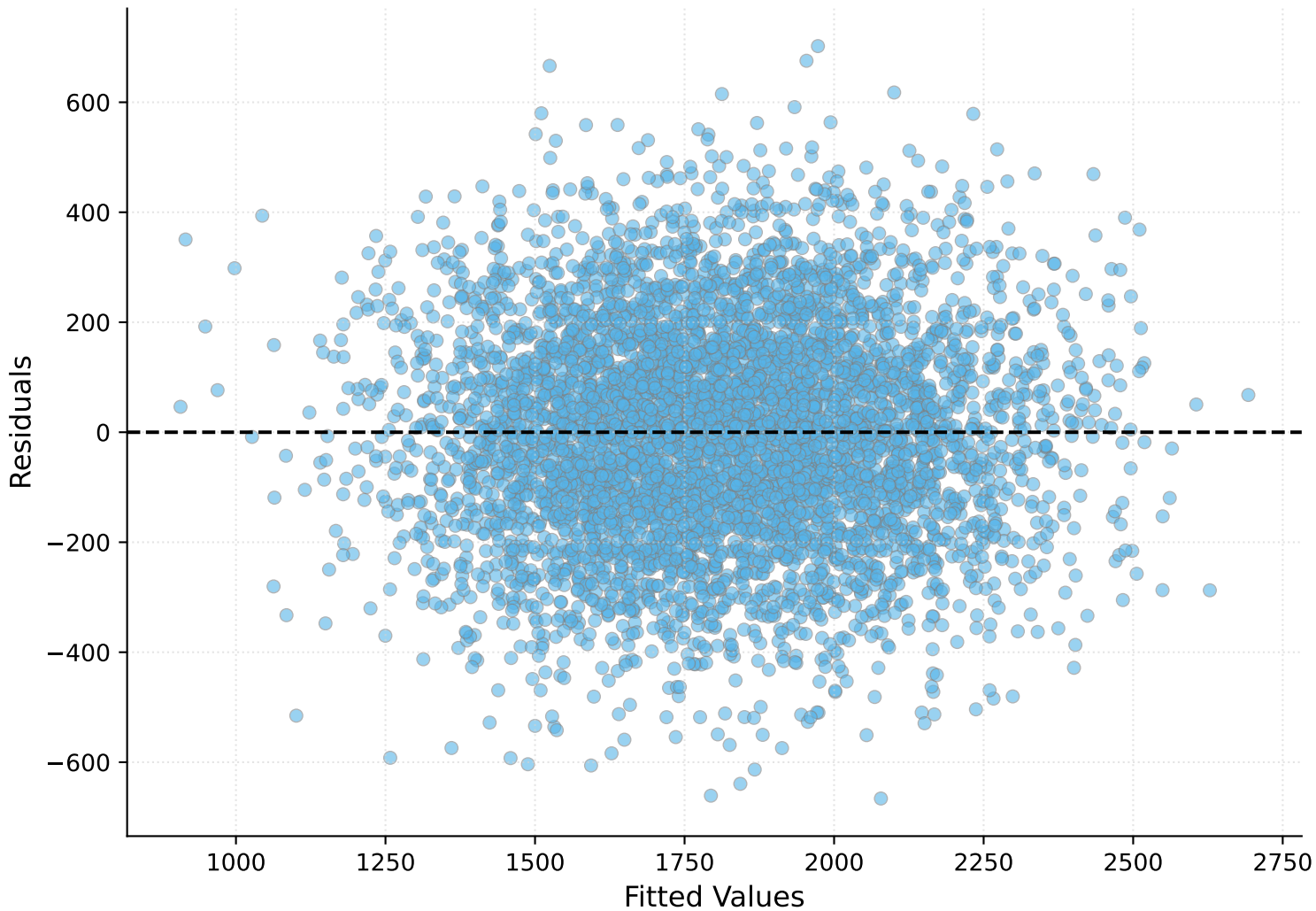
Residuals vs. Fitted Values (LRE)
