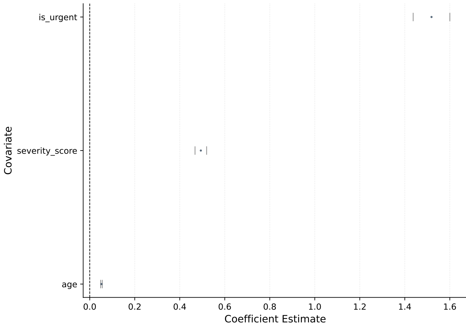
Forest Plot of Covariate Effects (Beta) on Length of Stay
