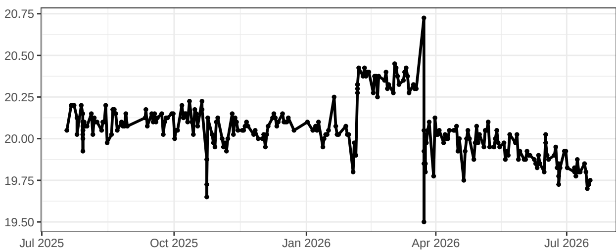
UV-Laser Power
