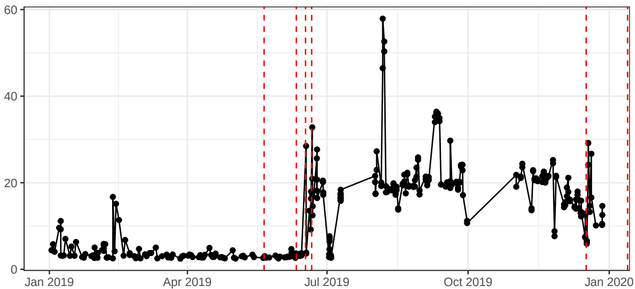
SSC-W-% rCV
