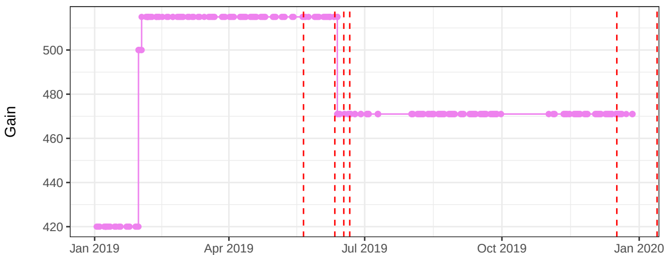
V525-A_Gain
