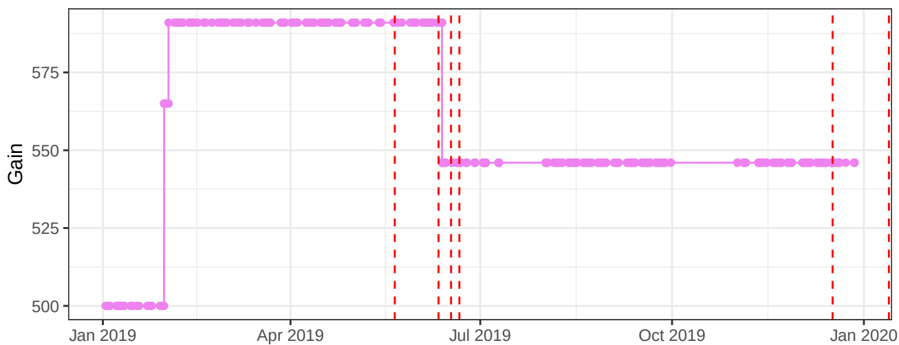
V670-A_Gain
