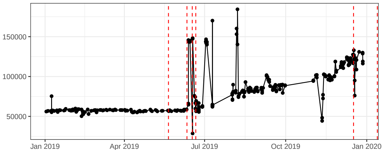
V450-A_Gain
