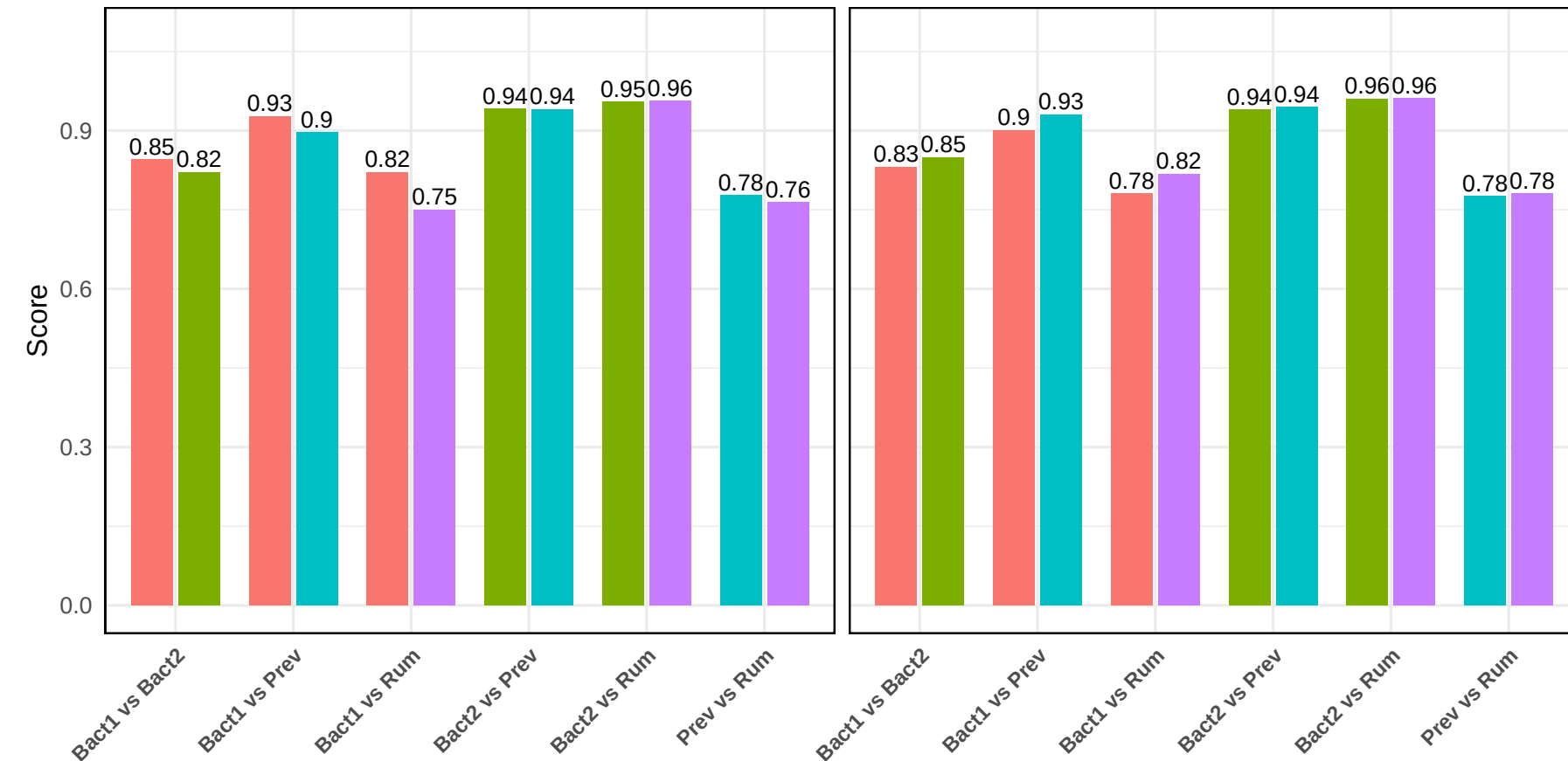
Recall
