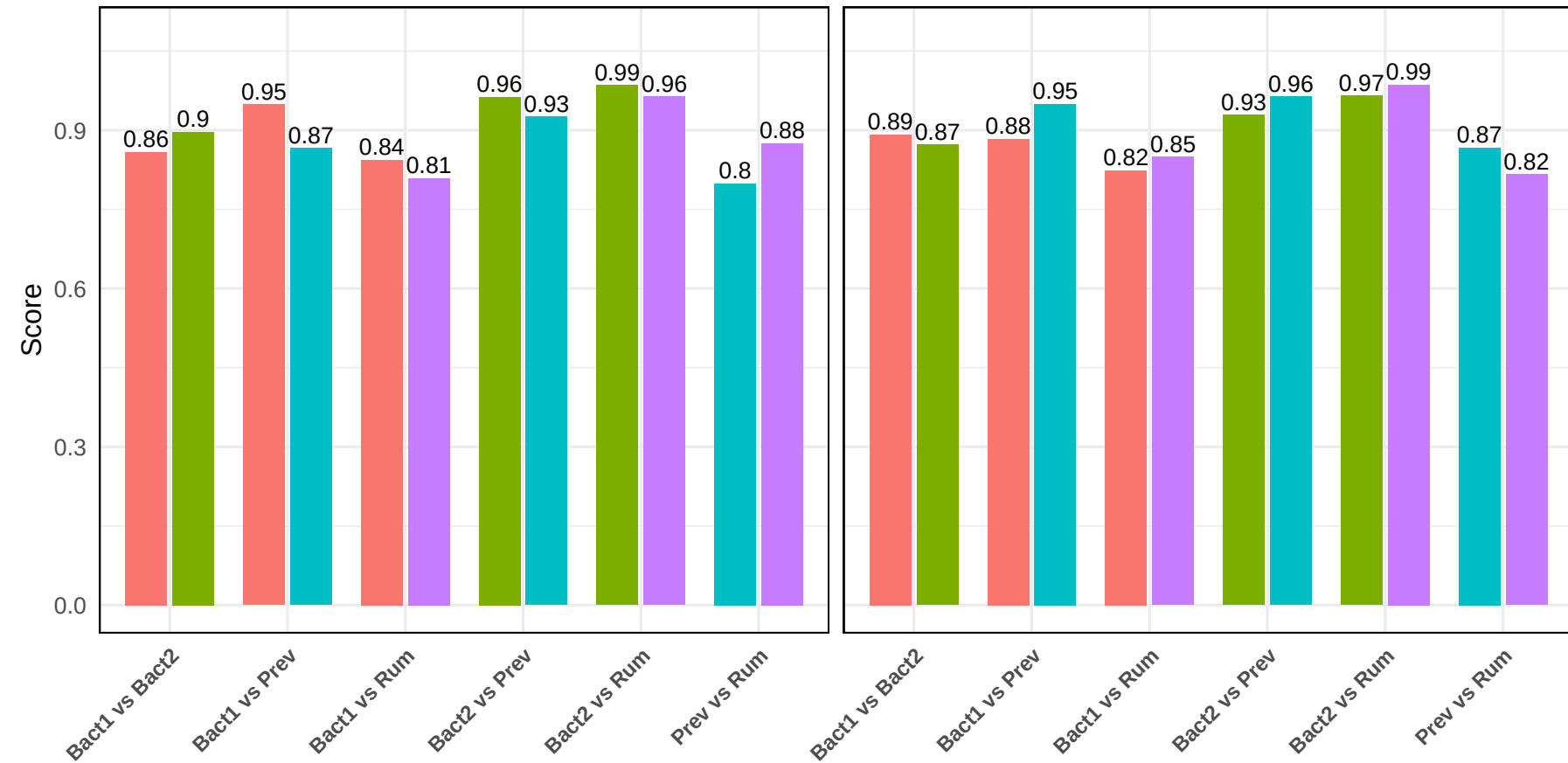
Logistic Regression
